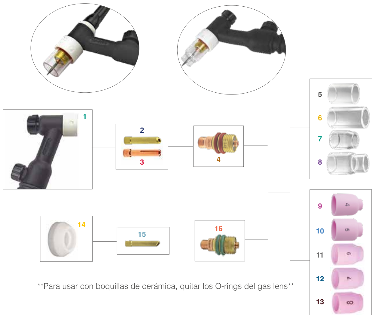
BOQUILLA RECTA
